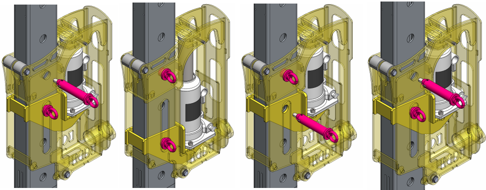
Figure 6 Climber unit pin sequence.
